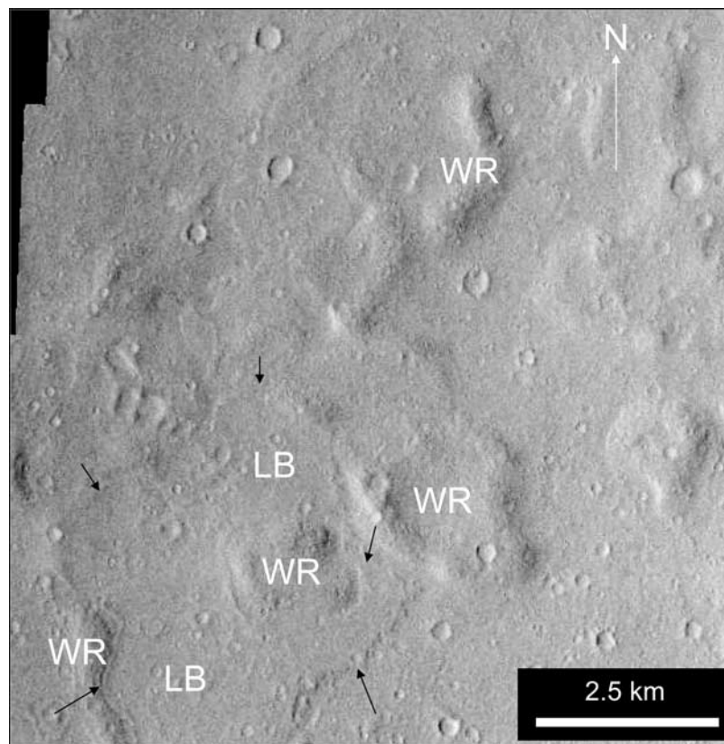
Figure 18. LB deposited against and between ridges of WR in north central Gusev (THEMIS-V-01580003).
