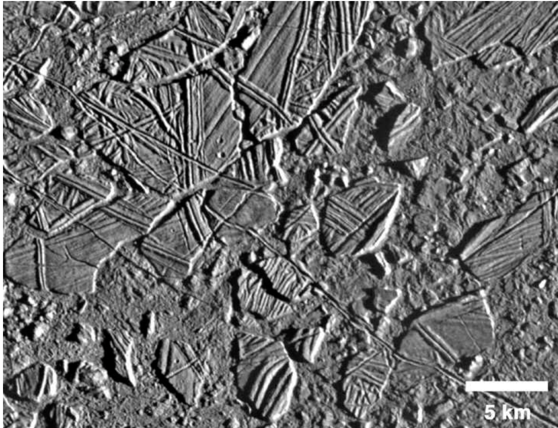
Figure 1.6: High-resolution view of the interior of a chaos region on Europa. Blocks of existing terrain have rotated, translated, and re-frozen in hummocky-textured matrix material. (Image PIA00591.)
