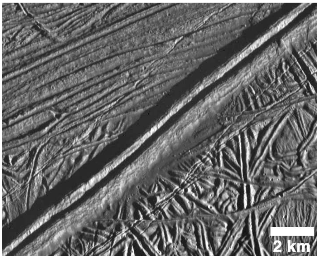
Figure 1.4: High resolution (20 meters per pixel) image of a double ridge approximately 2 km wide on the surface of Europa. Pre-existing terrain is preserved on the upwarped flanks of the ridge, lending support to the hypothesis that uplift, potentially from thermal buoyancy, drives ridge formation. (Image PIA00589.)
