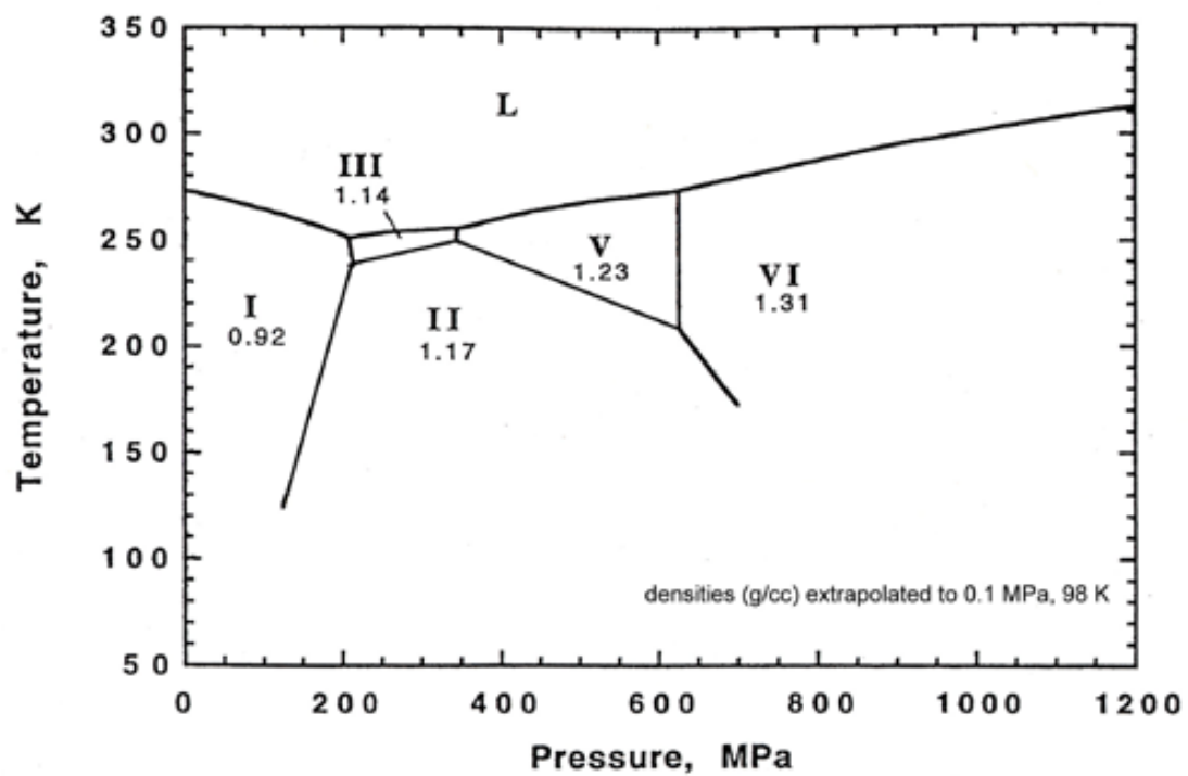
Figure 1.2: Phase diagram for water ice, and associated densities in \text{g cm}^{-3} after Durham et al. (1997). L stands for liquid water.
