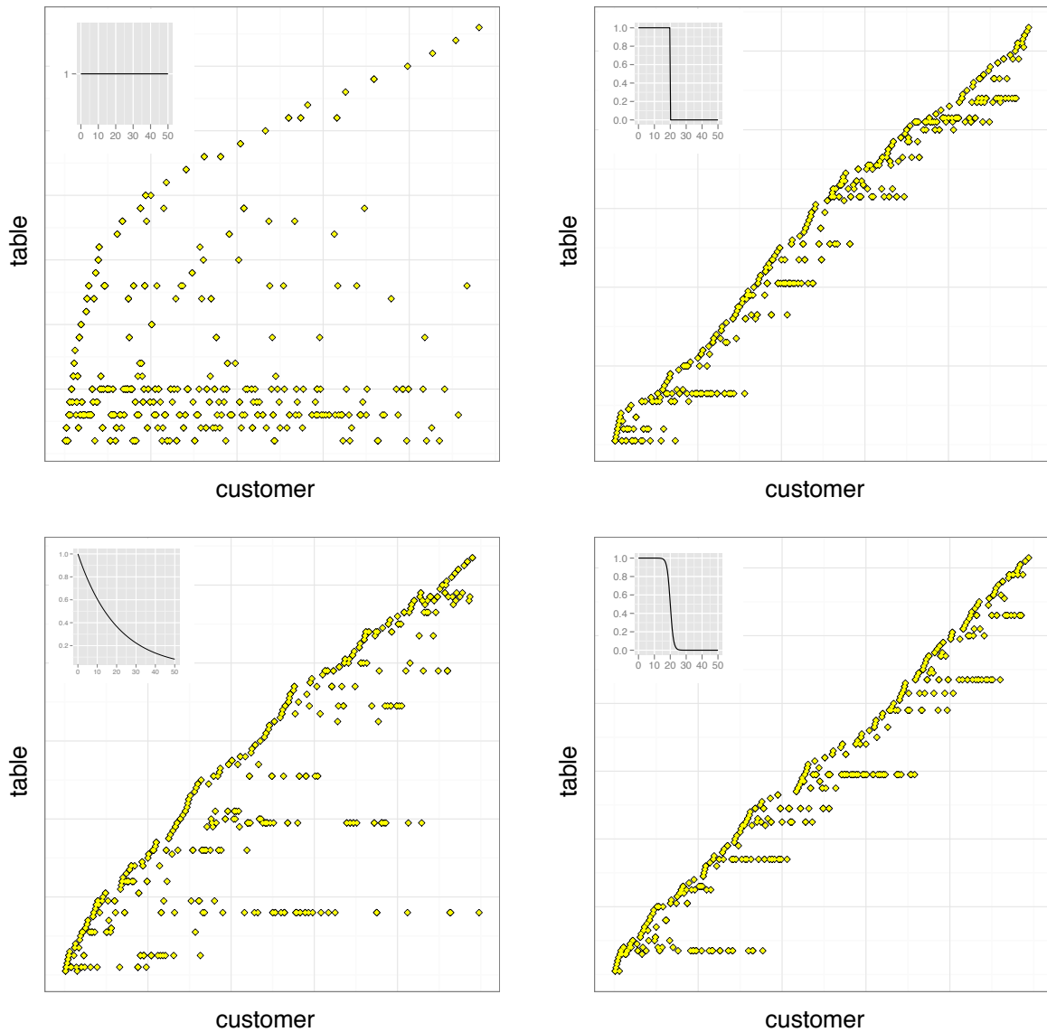
Figure 2: Draws from sequential CRPs. Illustrated are draws for different decay functions, which are inset: (1) The traditional CRP; (2) The window decay function; (3) The exponential decay function; (4) The logistic decay function. The table assignments are illustrated, which are derived from the customer assignments drawn from the distance dependent CRP. The decay functions (inset) are functions of the distance between the current customer and each previous customer.
