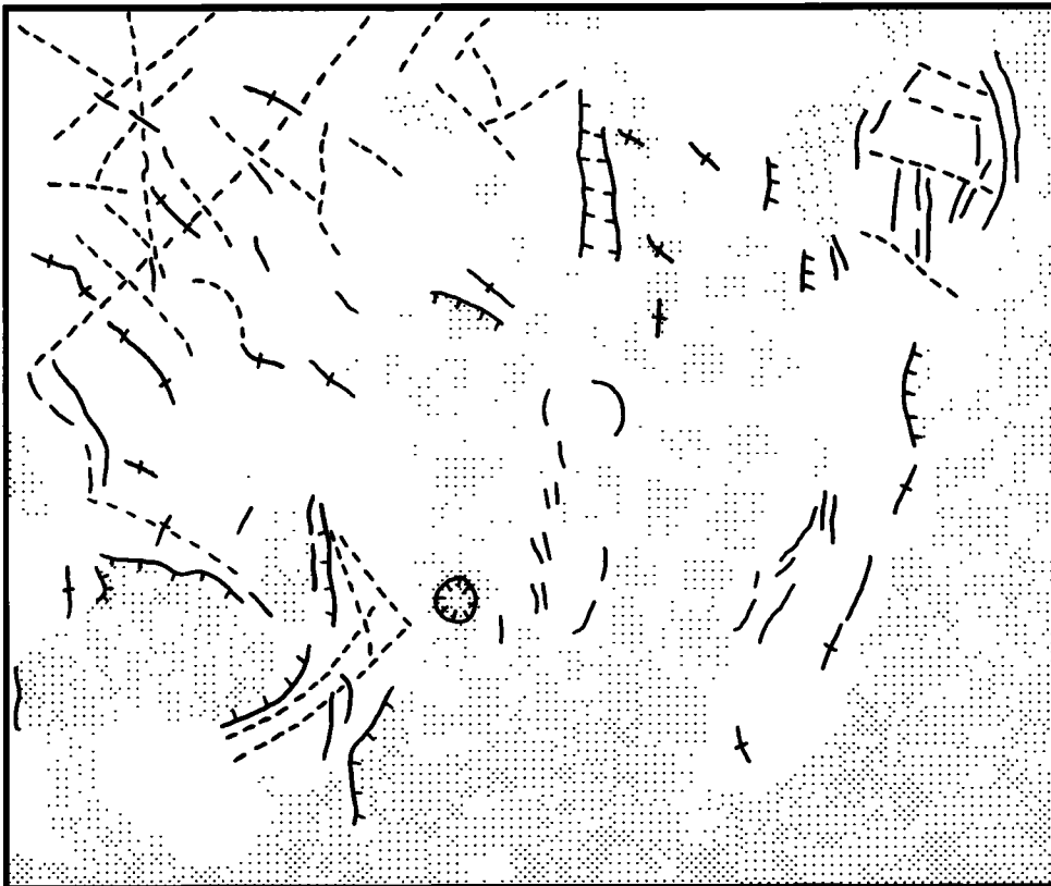
Fig. 6b. Sketch map of the region in Figure 6a. Structural symbols are the same as those used in Figure 5b. The stippled pattern represents plains regions.
