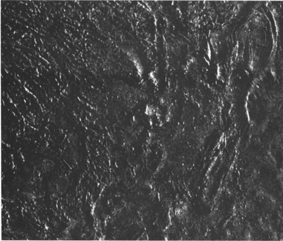
Fig. 6a. Venera image of type I boundary between tessera terrain and surrounding plains, located in southeastern Tellus Regio. Image is approximately 600 km E-W by 500 km N-S and is centered on 32.5°N, 85°E. Note the subdued appearance of tessera structures near the boundary, particularly in the upper central part of the image.
