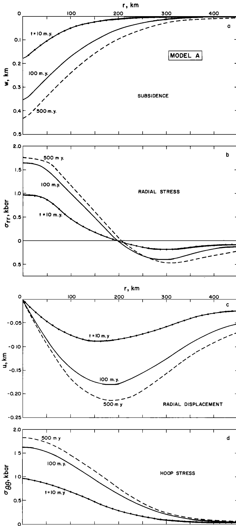
Fig. 11. Displacements and thermal stresses at the basin surface for model A (Figure 10). Curves shown represent accumulated values at 10, 100, and 500 m.y. after basin formation. (a) Subsidence w ; (b) radial stress \sigma_{rr} ; (c) radial displacement u , and (d) azimuthal or hoop stress \sigma_{\theta\theta} .
