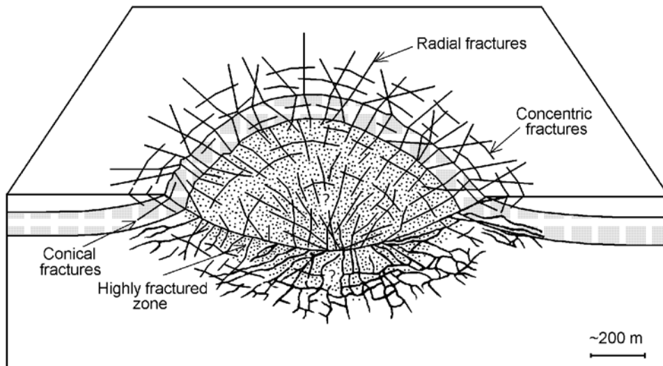
Figure 5. A schematic diagram showing the crater wall fractures.
