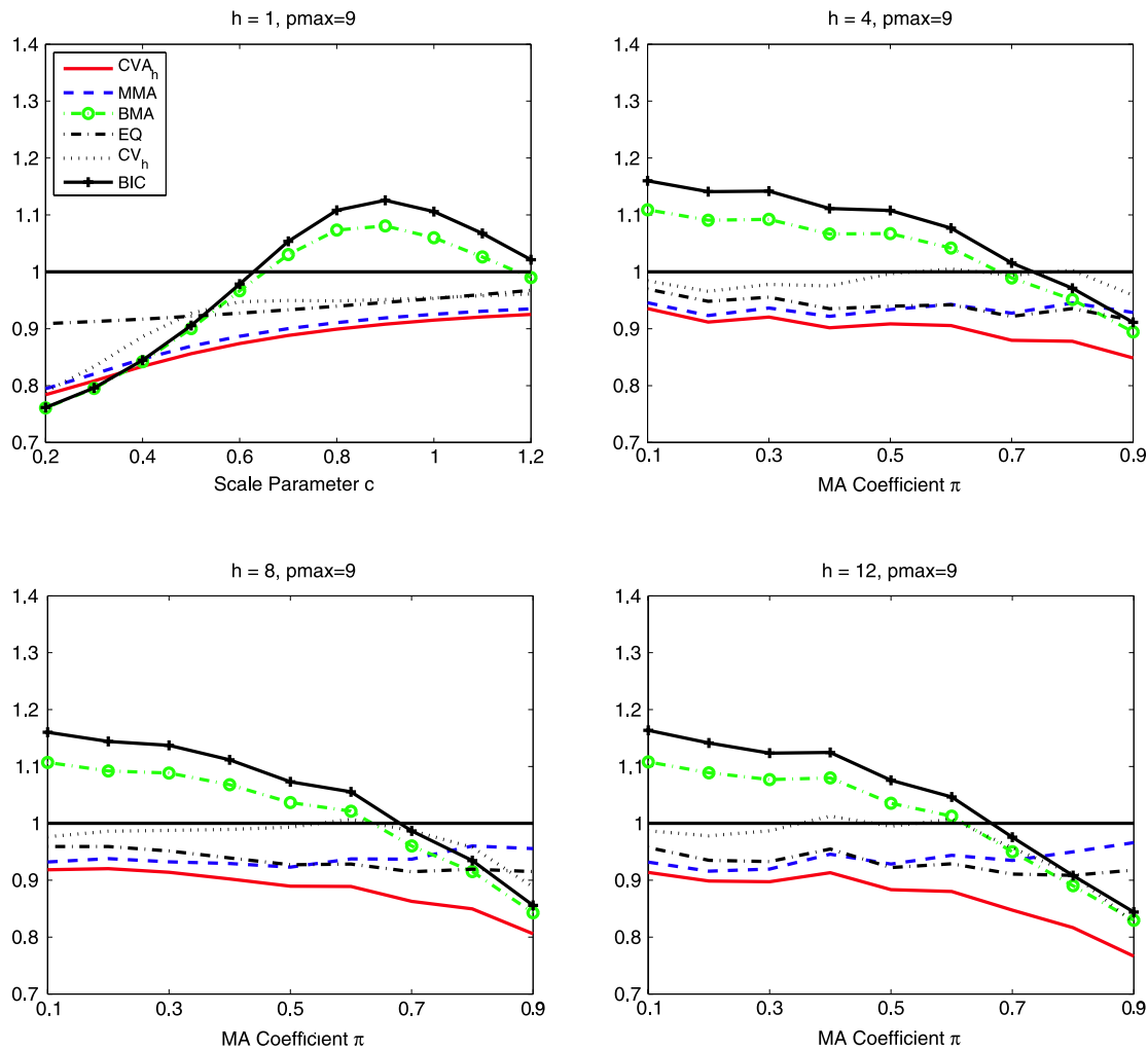
Fig. A.4. Relative MSFE for h = 1, 4, 8, and 12 when p_{\max} = 9 . The normalization is the same as in Fig. 1. CVA_h is leave- h -out cross-validation averaging. MMA is Mallows model averaging. BMA is Bayesian model averaging. EQ is equal weight simple averaging. CV_h is model selection with leave- h -out cross-validation. BIC is model selection with Bayesian information criterion.
