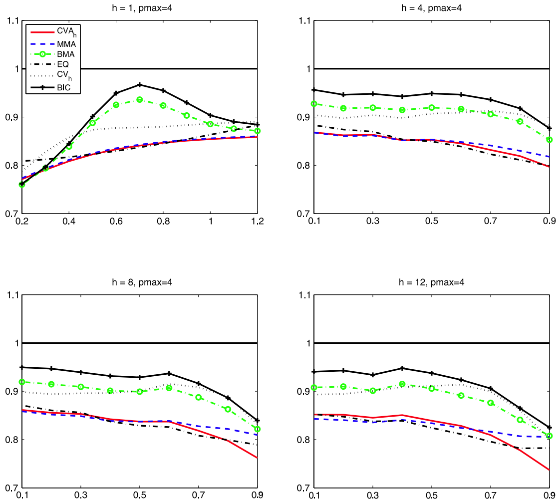
Fig. A.3. Relative MSFE for h = 1, 4, 8, and 12 when p_{max} = 4 . The normalization is the same as in Fig. 1. CVA_h is leave- h -out cross-validation averaging. MMA is Mallows model averaging. BMA is Bayesian model averaging. EQ is equal weight simple averaging. CV_h is model selection with leave- h -out cross-validation. BIC is model selection with Bayesian information criterion.
