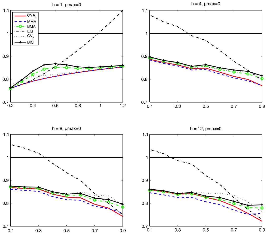
Fig. A.1. Relative MSFE for h = 1, 4, 8, and 12 when p_{\max} = 0 . (No lags of y_t and \tilde{F}_t are used.) The normalization is the same as in Fig. 1. CVA_h is leave- h -out cross-validation averaging. MMA is Mallows model averaging. BMA is Bayesian model averaging. EQ is equal weight simple averaging. CV_h is model selection with leave- h -out cross-validation. BIC is model selection with Bayesian information criterion.
