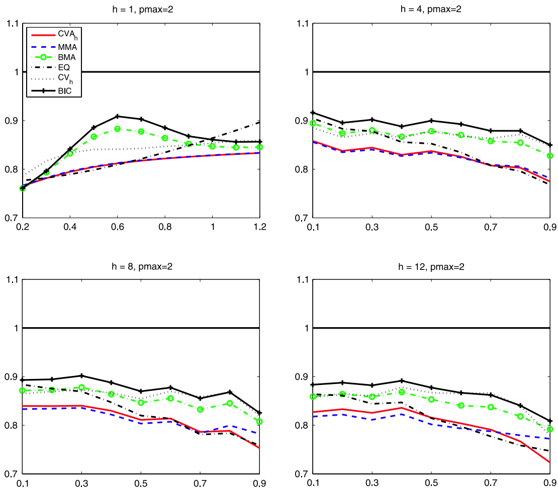
Fig. A.2. Relative MSFE for h = 1, 4, 8, and 12 when p_{\max} = 2 . The normalization is the same as in Fig. 1. CVA_h is leave- h -out cross-validation averaging. MMA is Mallows model averaging. BMA is Bayesian model averaging. EQ is equal weight simple averaging. CV_h is model selection with leave- h -out cross-validation. BIC is model selection with Bayesian information criterion.
