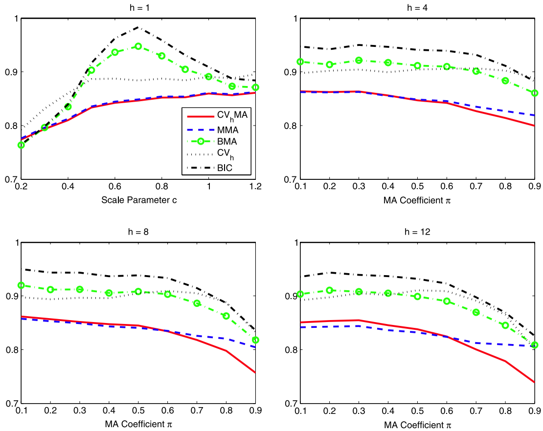
Fig. 1. Relative MSFE to least-squares forecast with all regressors for h = 1, 4, 8, and 12 . CVA_h is leave- h -out cross-validation averaging. MMA is Mallows model averaging. BMA is Bayesian model averaging. CV_h is model selection with leave- h -out cross-validation. BIC is model selection with Bayesian information criterion.
