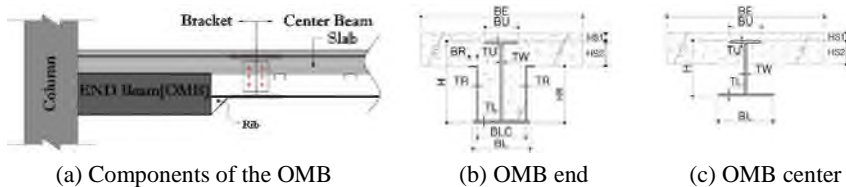
Fig.3 OMB system
