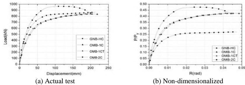
Fig. 5 P-\delta curves
