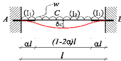
Fig. 1 OMB subjected to uniformly distributed load w
