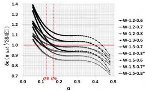
Fig.2 Variation in central deflection under uniformly distributed loads \omega
