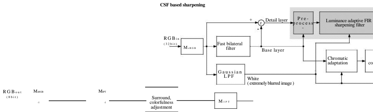
Fig. 2. The block diagram of the proposed method.
