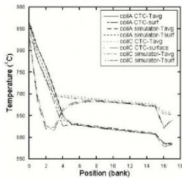
Fig.2. Temperature variations along the strip on ROT
