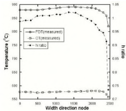
Fig. 3. Temperature and HTC distribution across the width direction
