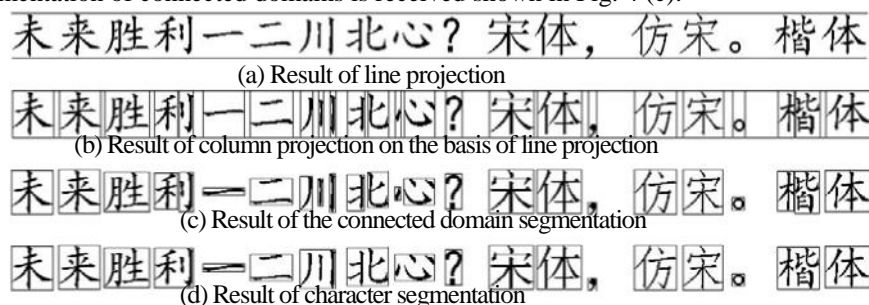
Fig. 4. Procedure of connected domain segmentation
