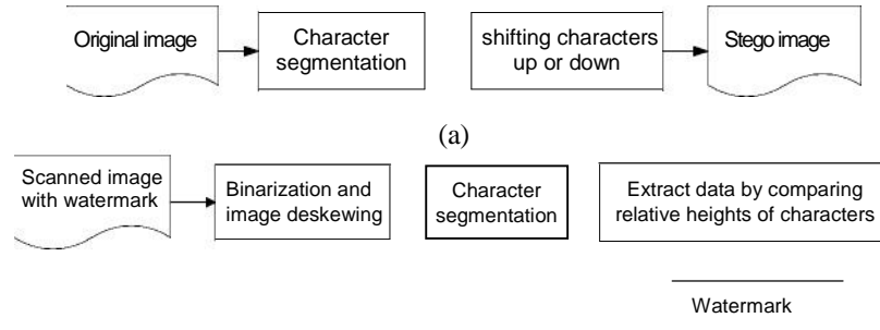
(a) Fig. 1. Framework of proposed methods, (a) Watermark embedding, (b) Watermark extracting
