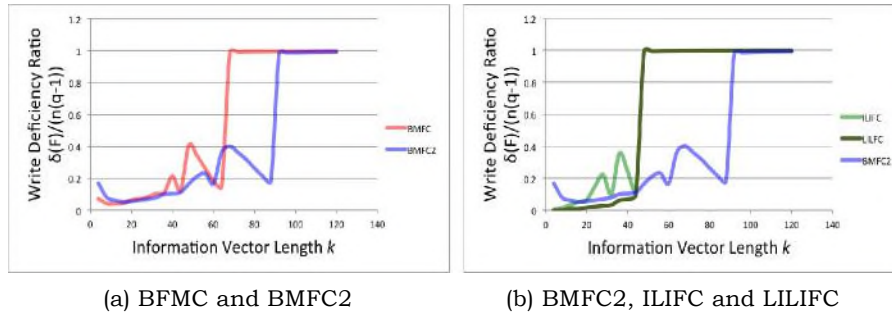
Fig. 2: Average Write Deficiency Ratios of BMFC, BMFC2, ILIFC and LILIFC in Uniform Frequency Distribution
