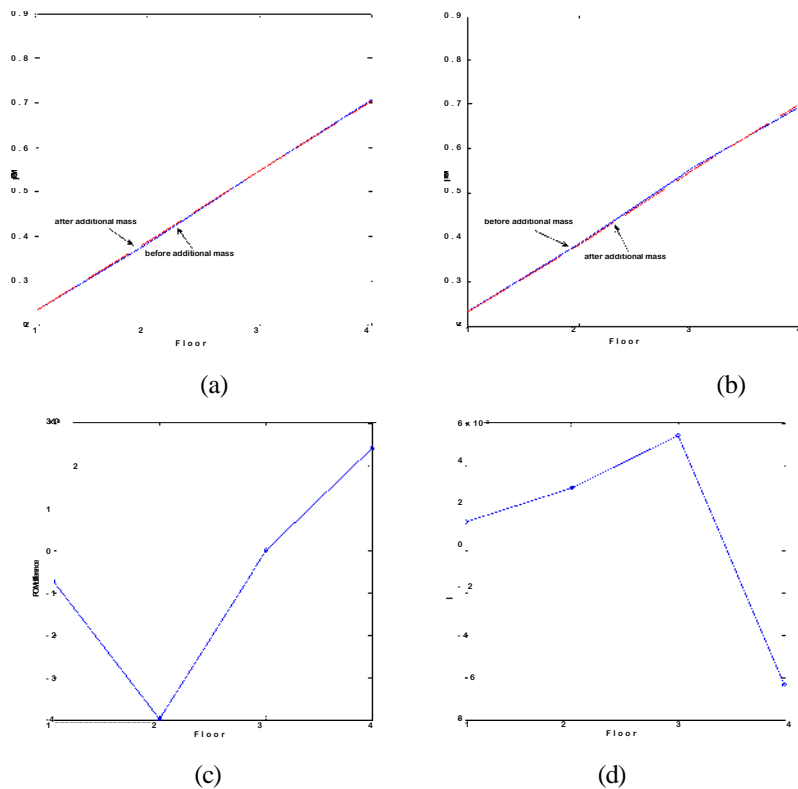
Fig. 4. POM and its difference between two states (uniform mass distribution): (a) POM (damage at the second floor), (b) POM (damage at the fourth floor), (c) POM difference (damage at the second floor), (d) POM difference (damage at the fourth floor)
