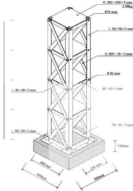
Fig. 1. Four-story steel frame structure.
