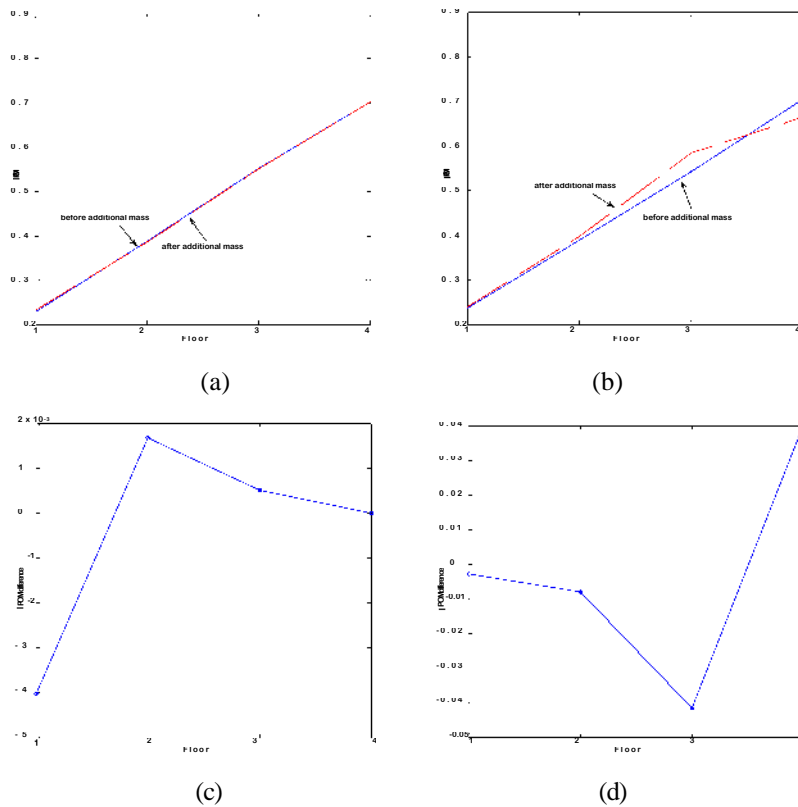
Fig. 5. POM and its difference between two states (nonuniform mass distribution): (a) POM (damage at the second floor), (b) POM (damage at the fourth floor), (c) POM difference (damage at the second floor), (d) POM difference (damage at the fourth floor)
