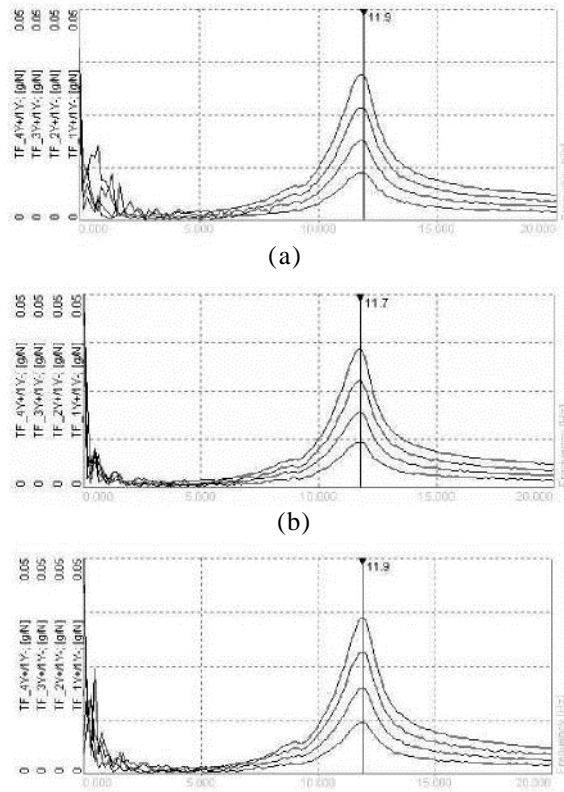
(b) Fig. 3. Curves of FRF magnitude of the building model: (a) before placing the additional mass, (b) after placing the additional mass at the second floor, (c) after placing the additional mass at the fourth floor
