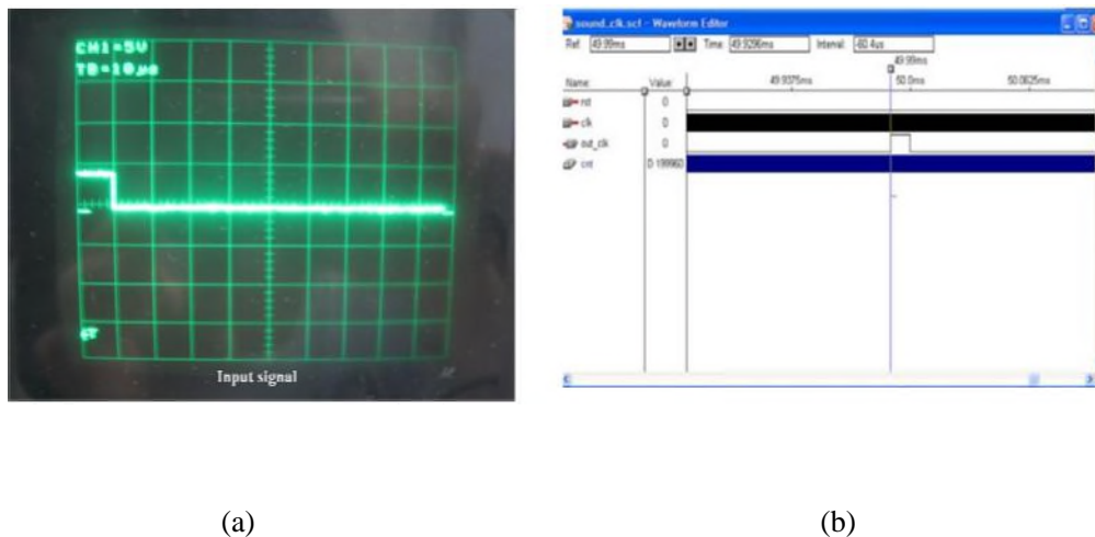
Figure 2. (a)Sensor input signal with 10 \mu s in oscilloscope screen and (b) simulation result of input signal.
