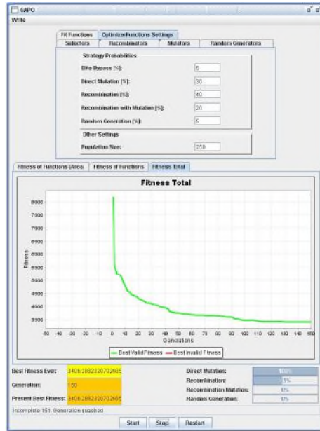
Fig. 2. Screenshot of GAPO's user interface
