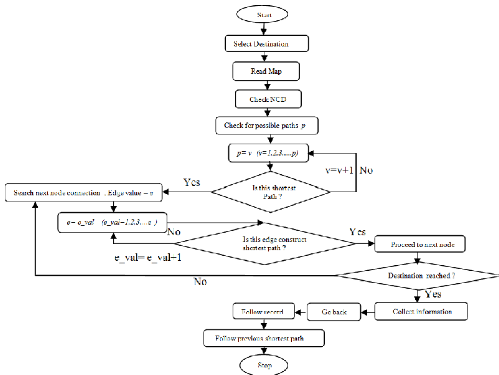
Figure 9. Shortest Path Algorithm (SPA) for Robot colony
