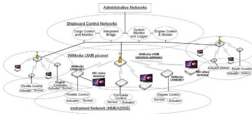
Fig. 2. WiMedia UWB based ship area pico-network supporting mixed video stream data and shipboard control data.
