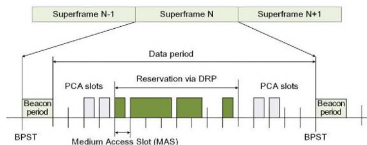
Fig. 1. The structure of channel allocation with WiMedia MAC protocols such as DRP and PCA.
