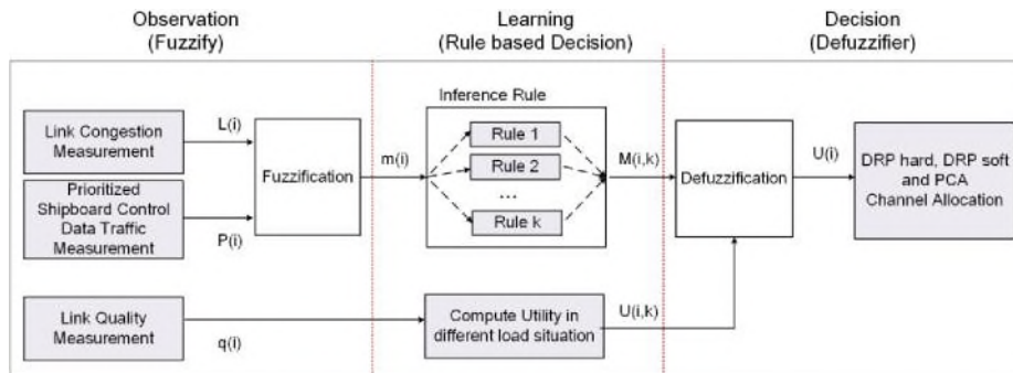
Fig. 3. Fuzzy logic control based dynamic channel allocation scheme
