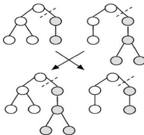
Figure 3. Example of the Crossover Operator
