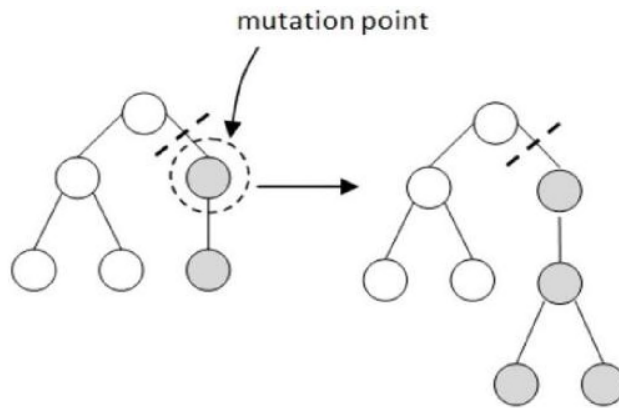
Figure 4. Example of the Mutation Operator
