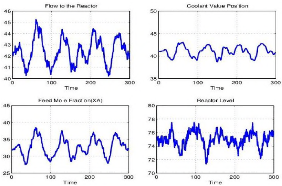
Figure 5. Input/Output Data for the Reactor Level Model
